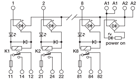
8 relay module
