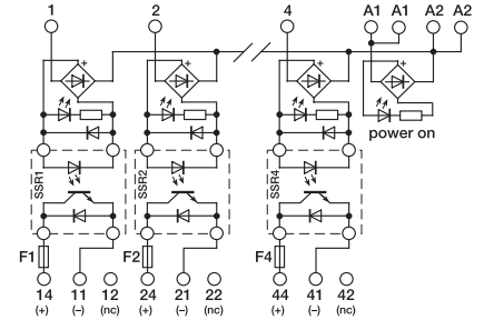
4 relay module
